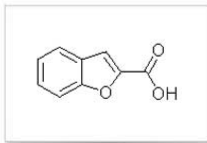
Benzofuran-2-Carboxylic Acid
