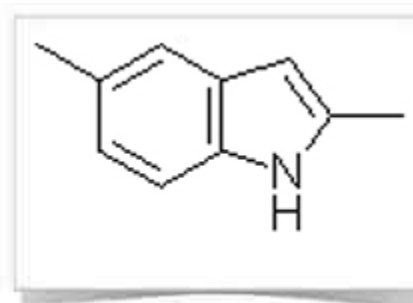
2,5-dimethylindole
