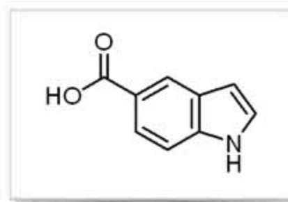
Indole-5-carboxylic acid
