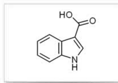
Indole-3-carboxylic acid
