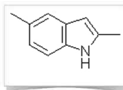
6-methylindole
