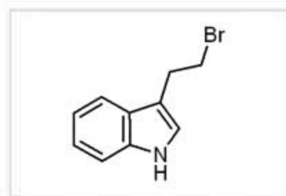
3-(2-Bromoethyl)Indole
