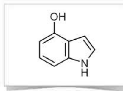
4-hydroxyindole
