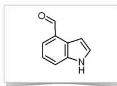
1H-Indole-4-carboxaldehyde
