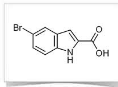
5-Bromoindole-2-carboxylic acid
