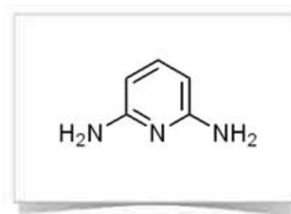
2,6-Diaminopyridine
