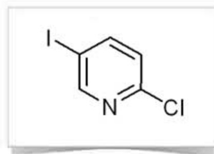
2-Chloro-5-iodopyridine
