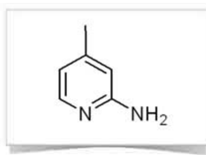
2-Amino-4-methylpyridine
