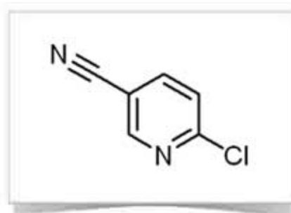
2-Chloro-5-cyanopyridine
