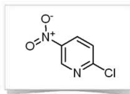
2-Chloro-5-nitropyridine
