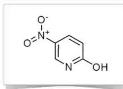
2-Hydroxy-5-nitropyridine
