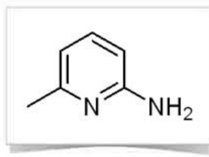
2-Amino-6-methylpyridine
