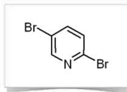
2,5-Dibromopyridine
