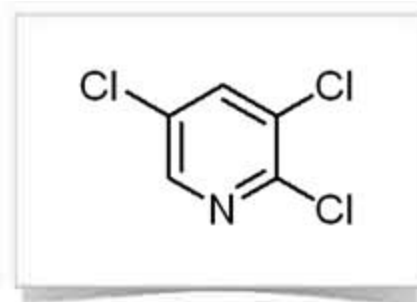
2,3,5-Trichloropyridine
