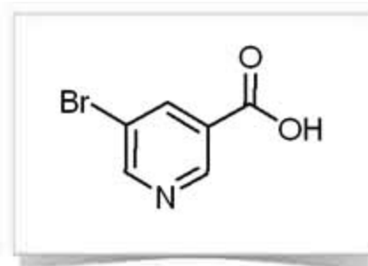
5-Bromo-3-carboxypyridine
