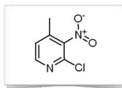
2-Chloro-4-methyl-3-nitropyridine
