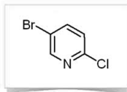
2-Chloro-5-bromopyridine
