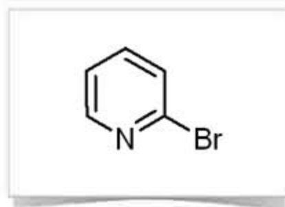
2-Bromopyridine
