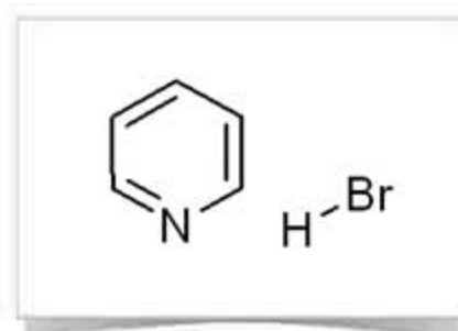
Pyridine hydrobromide
