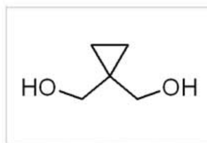
Cyclopropanedimethanol
