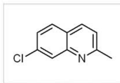
7-Chloroquinaldine
