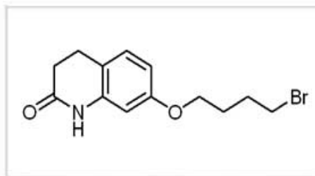
7-(4-Bromobutoxy)-3,4-dihydrocarbostyryl
