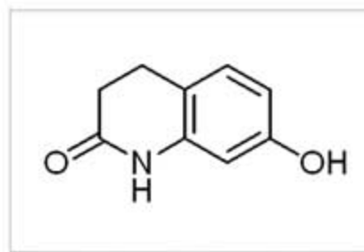
7-Hydroxy-3,4-dihydrocarbostyryl
