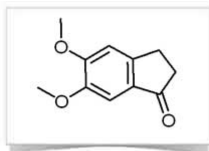
5,6-Dimethoxyindanone
