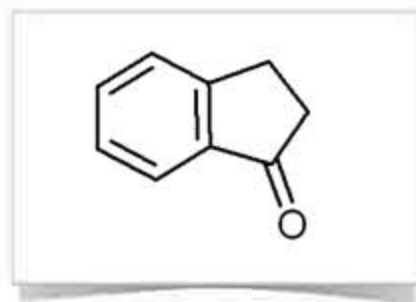
1-Indanone
