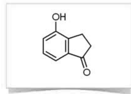
4-Hydroxy-1-indanone
