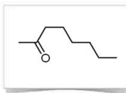
2-Octanone
