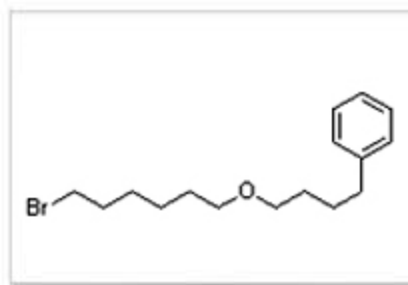
Salmeterol Intermediate
