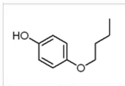
4-Butoxyphenol
