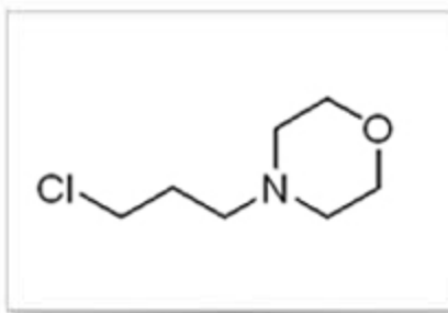
3-Morpholinopropyl chloride
