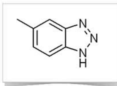
5-Methyl-1H-Benzotriazole
