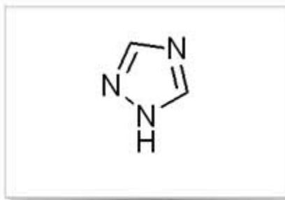
1,2,4-Triazole
