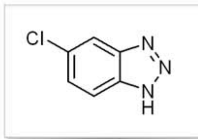
5-Chlorobenzotriazole
