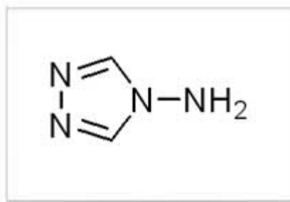
4-Amino-4H-1,2,4-Triazole
