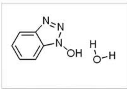
1-Hydroxybenzotriazole hydrate
